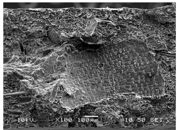
Fig. 7. Debonding of a very large soft particle and the catastrophic failure of the composite. The SEM micrograph was taken from fracture surface created in tensile testing. Fiber content: 20 vol%.
