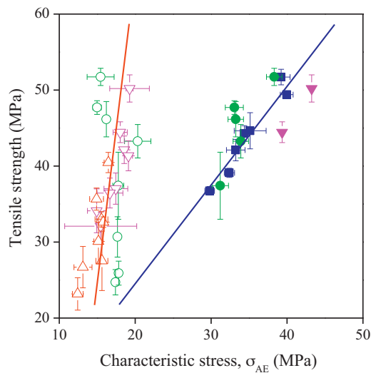
Fig. 6. Correlation between the characteristic stresses of the two micromechanical deformation processes detected by acoustic emission and the ultimate tensile strength of the composites. Symbols: (□) wood, (○) hard , (△) soft , (▽) gsoft ; empty symbol \sigma_{AE1} , full symbol \sigma_{AE2} .
