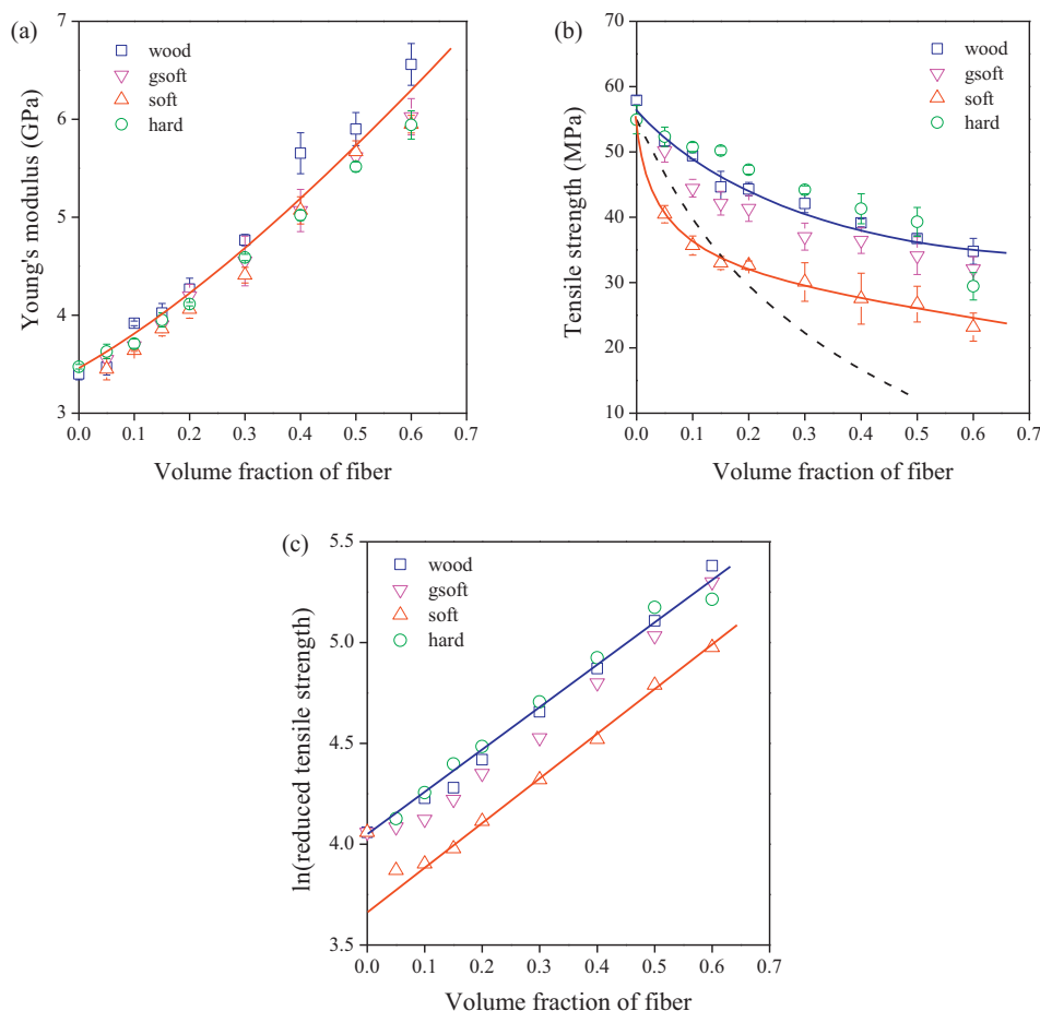
Fig. 4. Mechanical properties, reinforcement: (a) stiffness of PLA/lignocellulosic fiber composites plotted against fiber content. (b) Effect of the type and amount of reinforcement on the tensile strength of PLA/lignocellulosic fiber composites. ---- theoretical minimum of strength ( B=0 in Eq. (1)). (c) Reduced tensile strength of PLA/lignocellulosic fiber composites plotted against fiber content according to Eq. (2). Symbols: ( \square ) wood, ( \circ ) hard, ( \triangle ) soft, ( \nabla ) gsoft.
