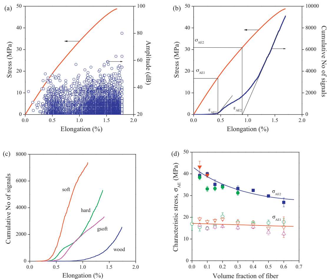
Fig. 3. Results of the acoustic emission measurements: (a) evolution of acoustic signals during the tensile testing of a PLA/wood composite (15 vol% heavy fraction); (o) individual acoustic signals, — stress vs. strain trace. (b) Cumulative number of signals vs. elongation trace of the composite of (a). The corresponding stress vs. strain trace is plotted as reference. Determination of characteristic stresses. (c) Comparison of the cumulative number of signal traces for all the PLA/lignocellulosic fiber composites studied; 15 vol% fiber content. (d) Composition dependence of the characteristic stresses derived from acoustic emission measurements; effect of fiber type. Symbols: ( \square ) wood, ( \circ ) hard, ( \triangle ) soft, ( \nabla ) gsoft; empty symbol \sigma_{AE1} , full symbol \sigma_{AE2} .
