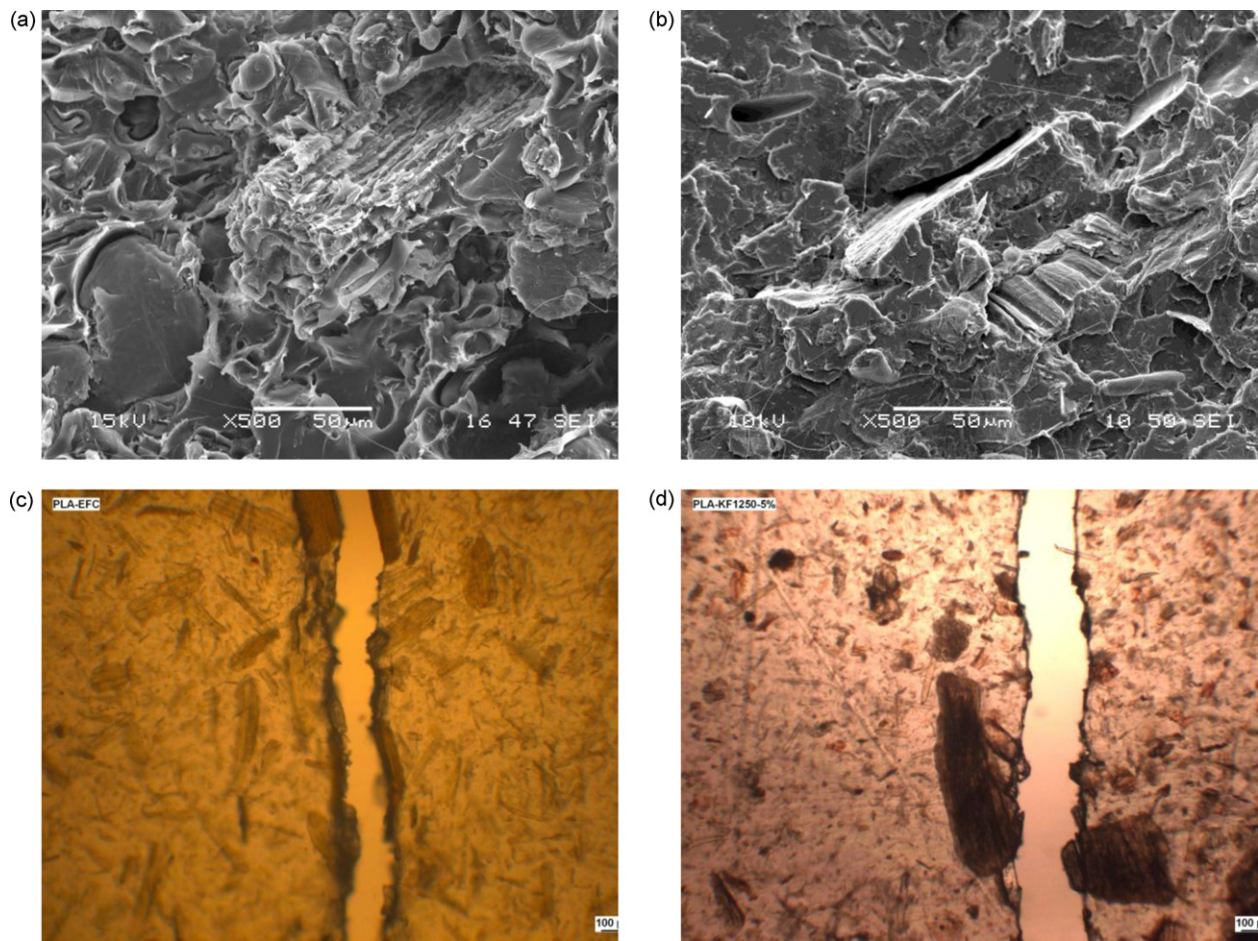
Fig. 5. Microscopy: (a and b) SEM micrographs taken from the fracture surface of a PLA/lignocellulosic fiber composites at 20 vol% fiber content. Fracture surface was created by failure in the tensile test: (a) hard and (b) ground soft particles . (c and d) Fiber fracture in PLA model composites, POM micrographs: (c) wood and (d) light fraction . The composites contained 5 vol% fiber.
